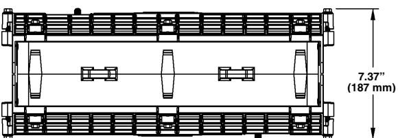
Dual Chamber Terminal Closure with 2 Standard Covers
