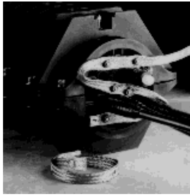
The Exterior Bond Braid bonds all isolated grounds together.
